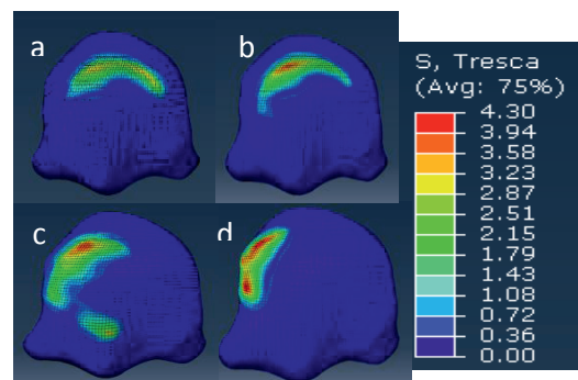
Figure 1: Shear stress in the 1st metatarsal cartilage for a) well-aligned toe, b) 10°, c) 20°, d) 30°
