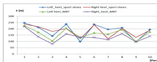
Figure 1: Comparison of forces under the calcaneus in MBT shoes and sport shoes (left and right)
