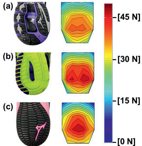
Figure 1: Force distribution across shoes: (a) standard shoe; (b) minimalist shoe with grooved heel pad; (c) minimalist shoe with curved heel pad.
