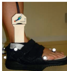
Figure 1: The WPS® talus shoe (Podartis, Treviso Italy) with a talus outsole equipped for the biomechanical evaluation.
