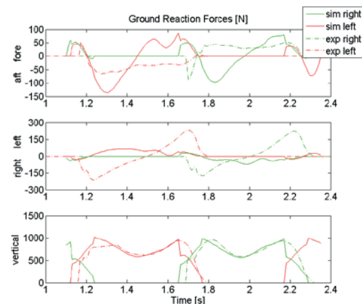
Figure 1: Simulated and experimental ground reaction forces in gait
